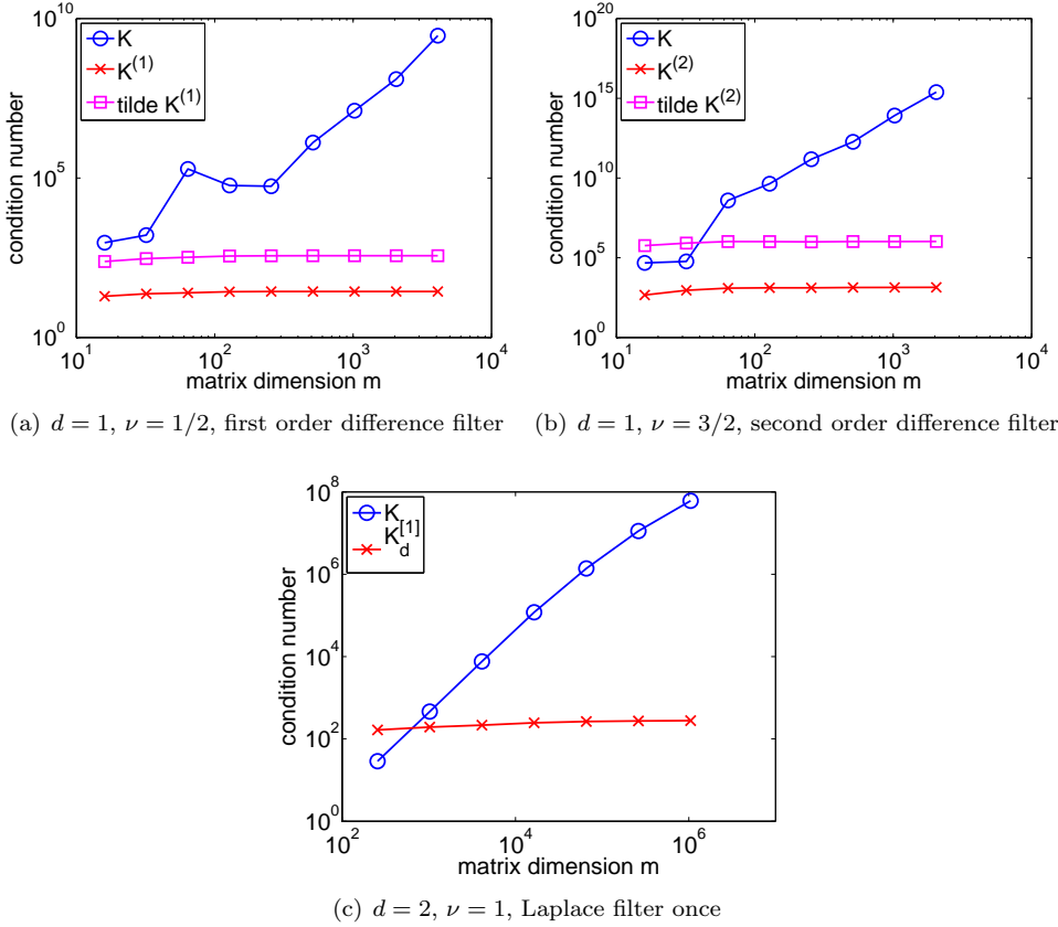
FIG. 4.1. Condition numbers of K (both unfiltered and filtered) as the matrix size varies.
