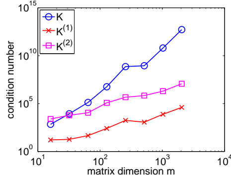
(b) d = 1, \nu = 1 , two filters
